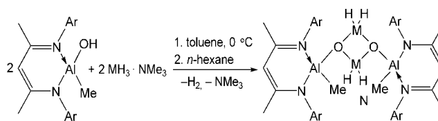
Scheme 1. Preparation of the tetranuclear alumoxane 2 (M = Al) and the gallium congener 3 (M = Ga); Ar = 2,6- i Pr 2 C 6 H 3 .
